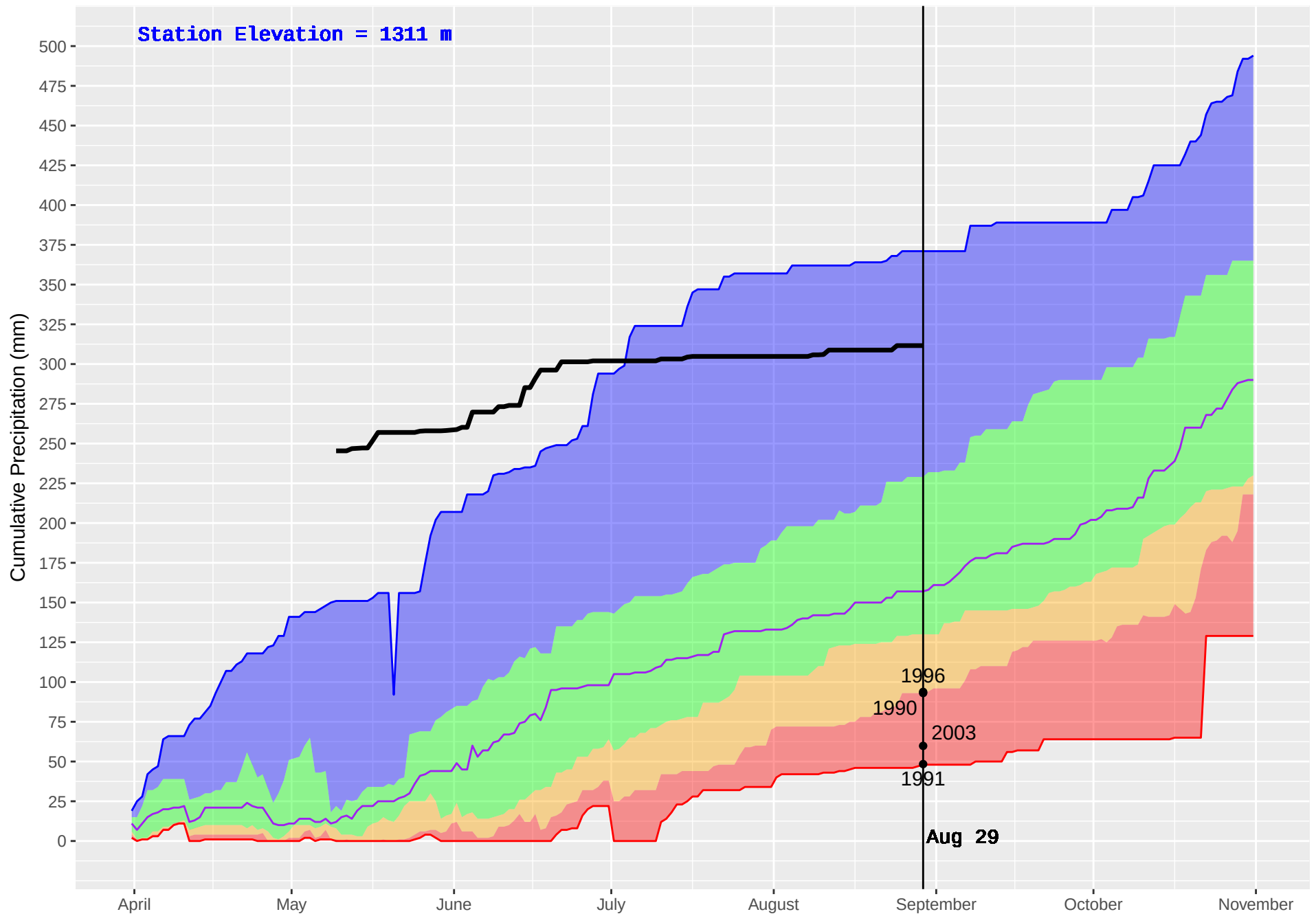
FLATHEAD 2 (418) : Historical (1986–2016) and Current (2017) Noon Cumulative Precipitation
